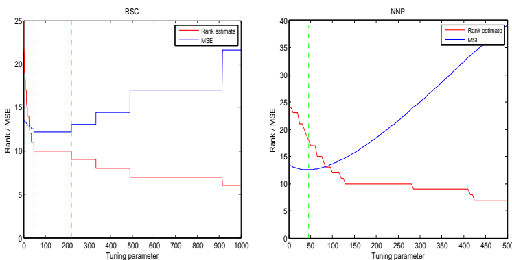
FIG 1. The MSE and rank of the estimators RSC (left) and NNP (right) as a function of the tuning parameter. The rank estimate and MSE curves are plotted together for a better view of the effect of tuning on different estimation aspects.
